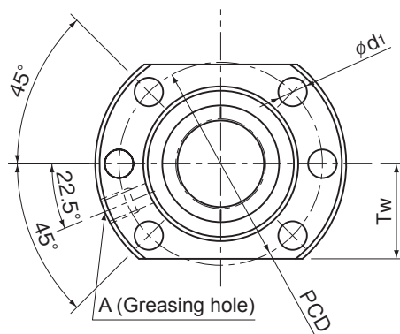
Hole type 1 (Model EPB1605 to 3210)
