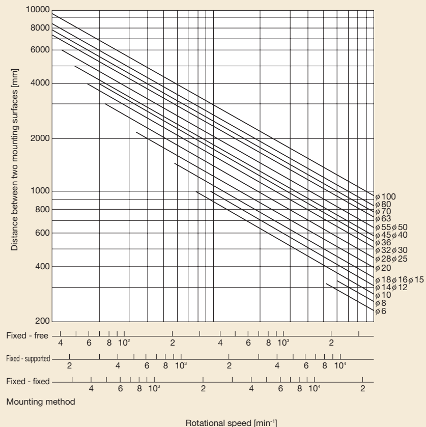
Fig.5 Permissible Rotational Speed Diagram
