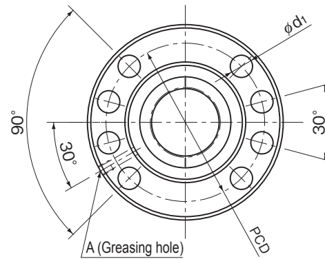
Hole type 2 (Model EBA4005 to 6320)
