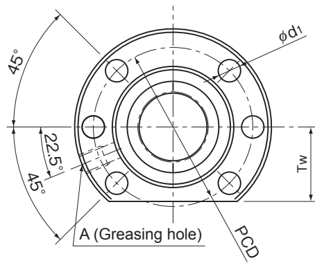
Hole type 1 (Model EBC1605 to 3210)
